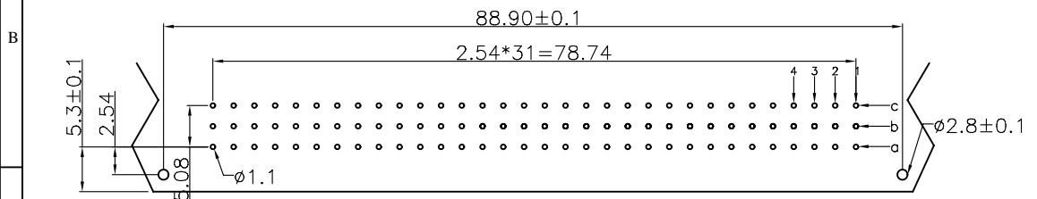
P.C.B Board Layout (Top Side) (PCB Tolerance ±0.05)
