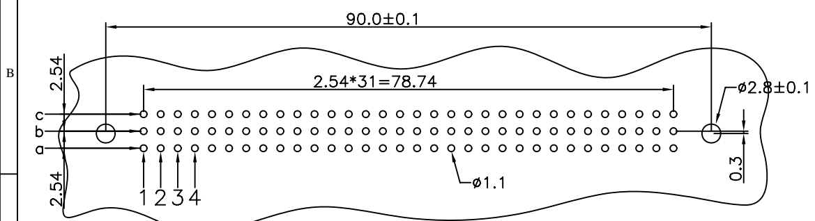
P.C.B Board Layout (Top Side) (PCB Tolerance ±0.05)
