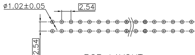
PCB LAYOUT
