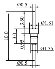
10.0mm PIN P/N0: P-127-1000-000-001
