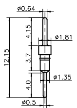
12.15mm PIN P/N0: P-127-1215-000-001
