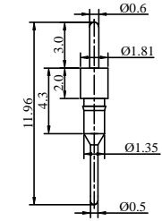
11.96mm PIN P/N0: P-127-1196-200-001
