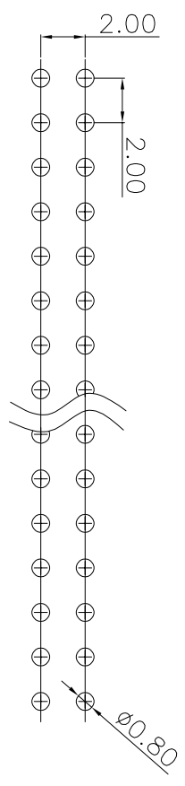
PCB LAYOUT
